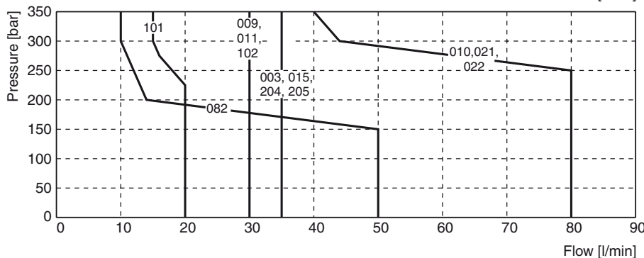
Measured with HLP46 at 50°C, 95% U nom and warm solenoids
