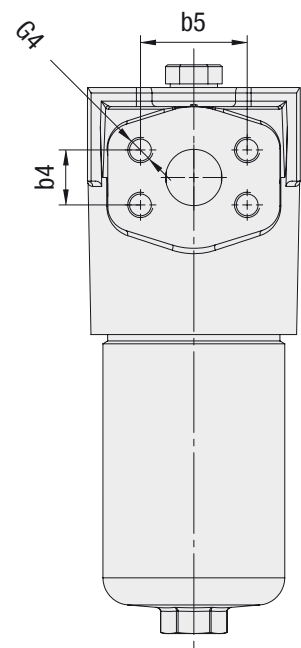
Flange connection
