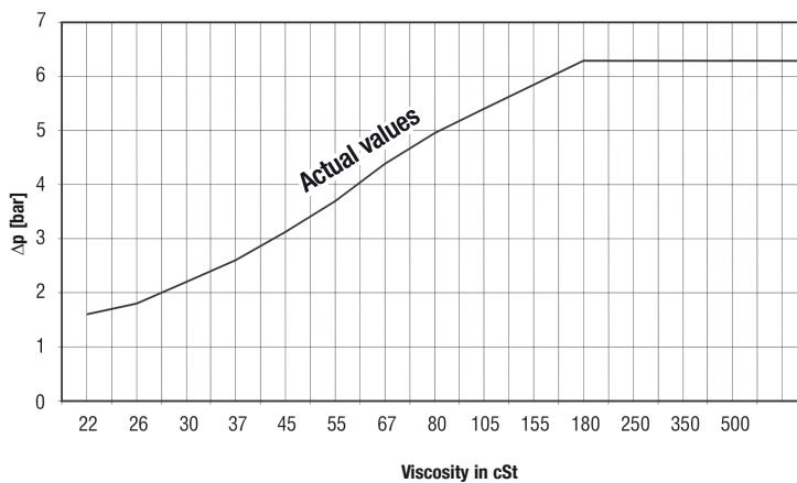
Filter Element SRM-30HB \Delta p / viscosity - graph
